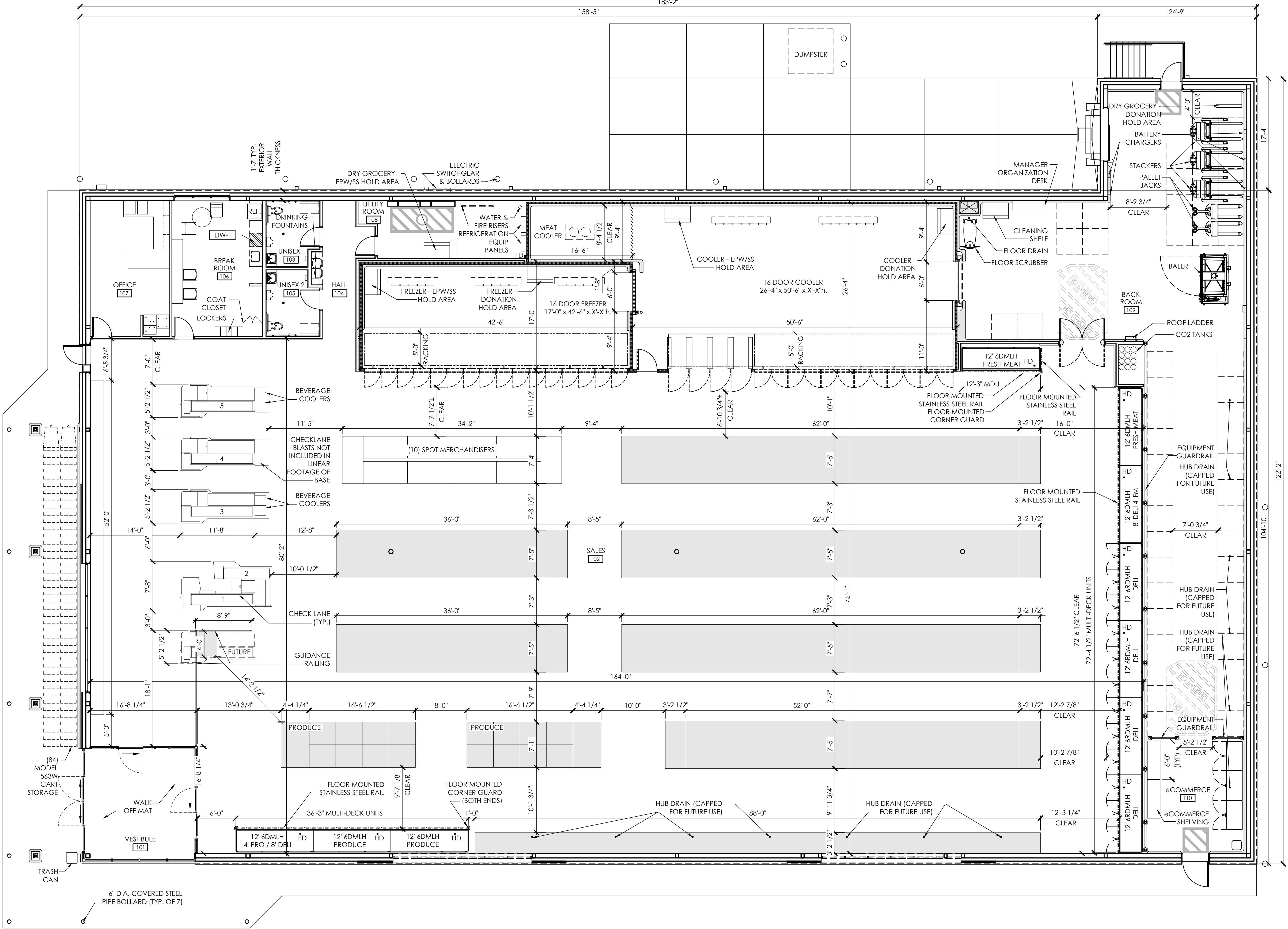
1 Operations Plan SCALE: 1/8" = 1'-0"
