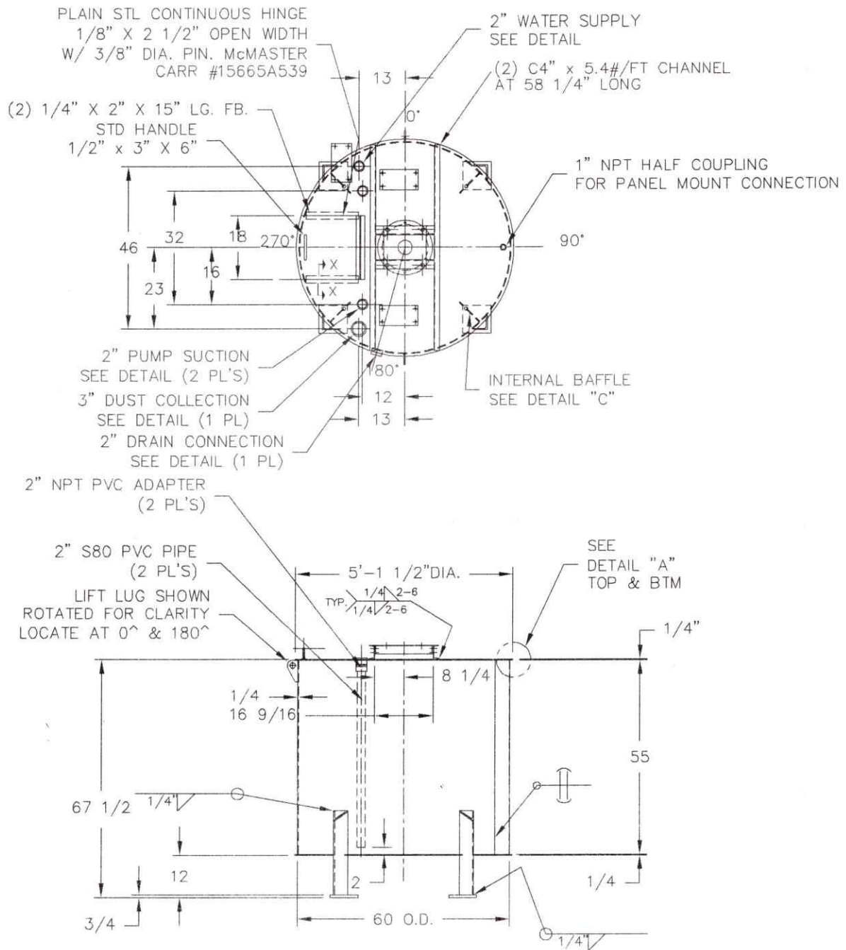
WELL #3 TANK
