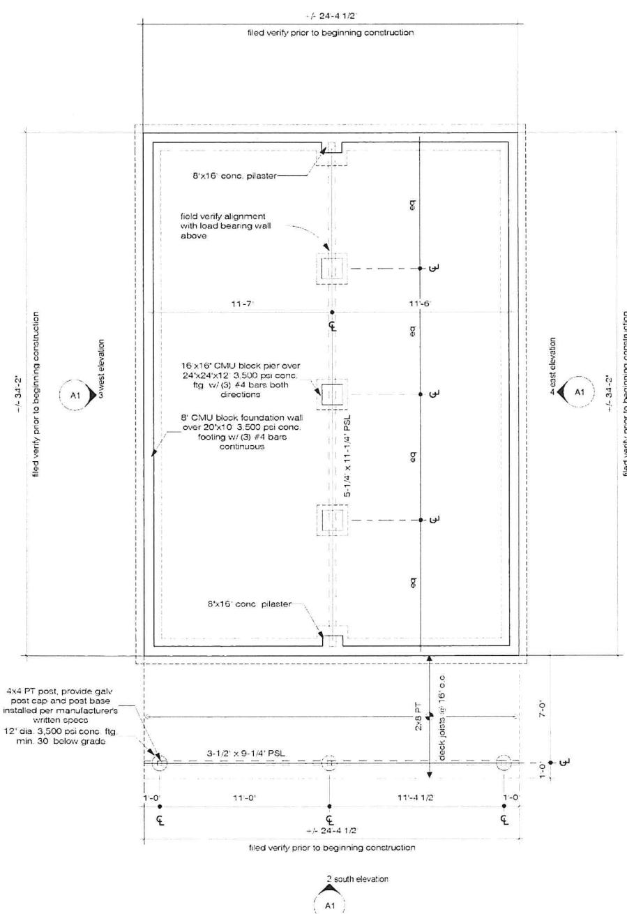
1 proposed foundation plan 1/4" = 1'-0"
