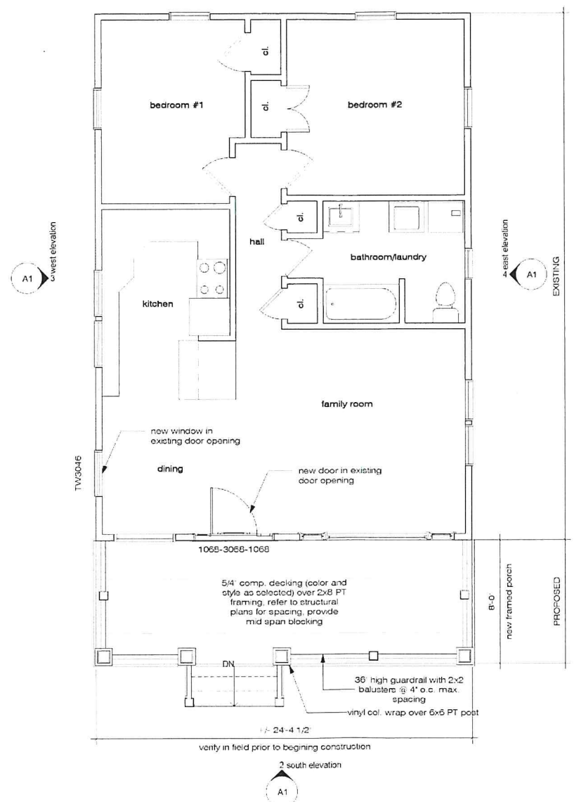
2 existing first floor and porch plan 1/4" = 1'-0"
