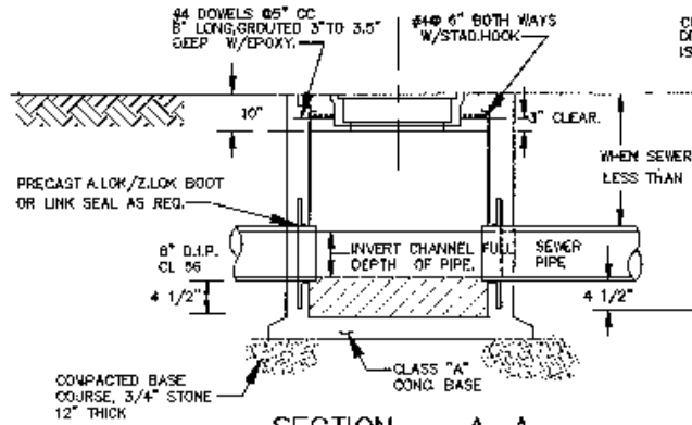
SECTION A-A SHALLOW MANHOLE
